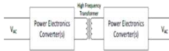
Fig. 1 Basic structure of SST
